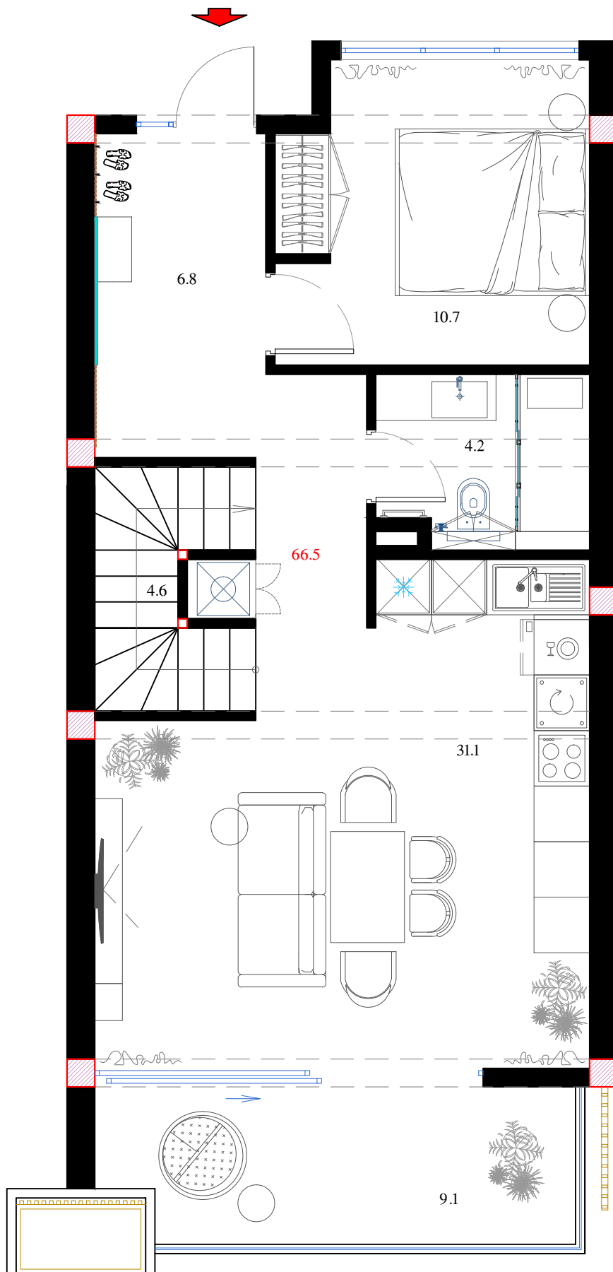
2 floor plan
