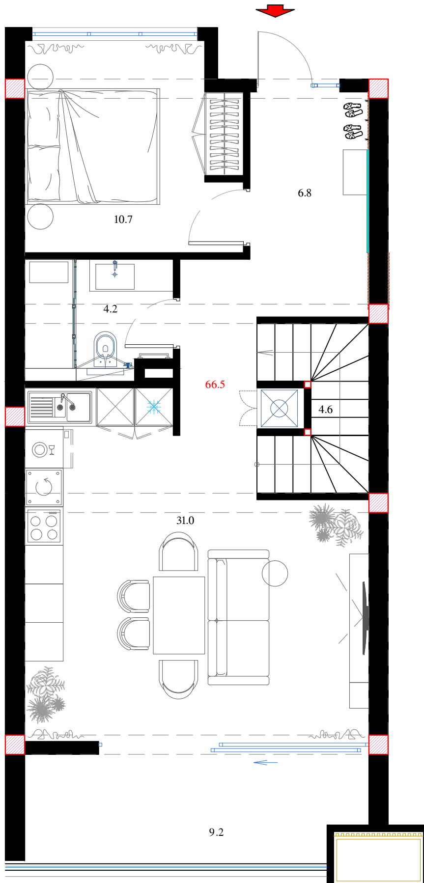
2 floor plan
