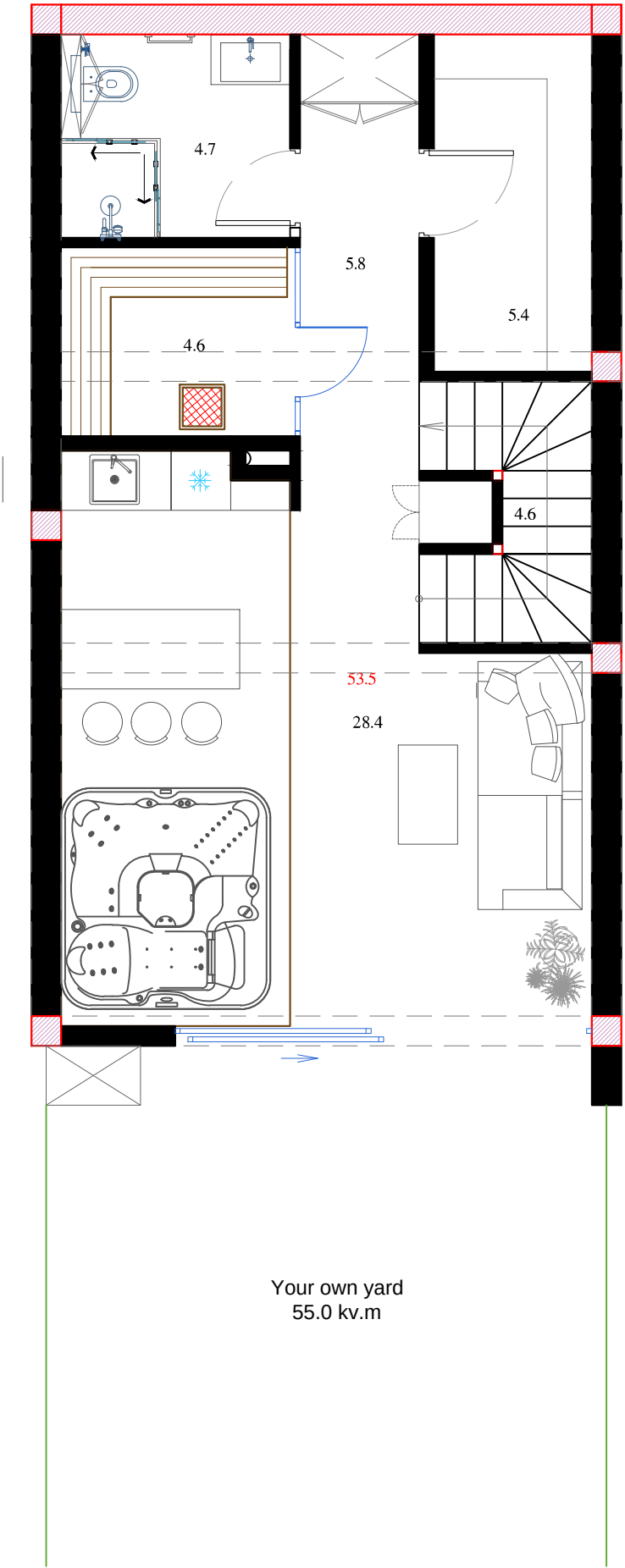
1 floor plan
