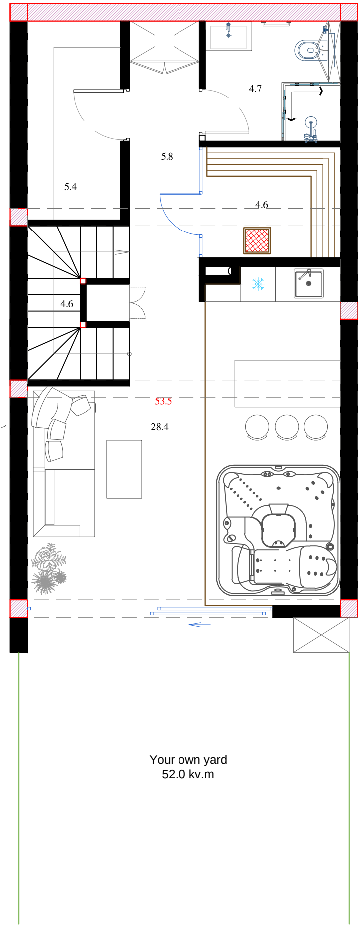
1 floor plan
